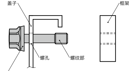
[SFHL-LH-SC-HD-E] 带法兰短头六角防脱落螺栓
