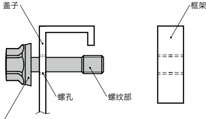
[SFHL-LH-SC-HP-HD-E] 带法兰短头六角防脱落螺栓
