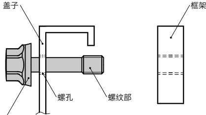
SFHL-LH-SC-HP-HD-H 带法兰短头六角防脱落螺栓
