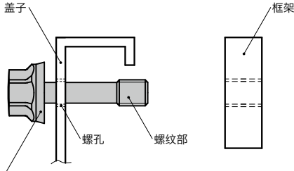
SFHL-LH-SC-HD-H 带法兰短头六角防脱落螺栓
