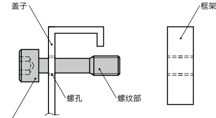
SSC-SNS-EL 内六角防脱落螺丝
